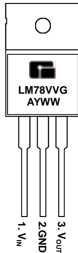
TO 220
