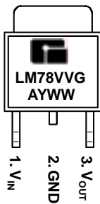
TO 252 (D-PAK)
